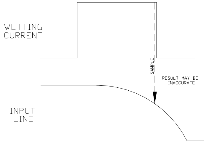
Figure-7 Example of Sampling Error due to Signal Distortion
