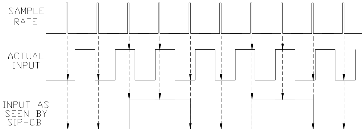
Figure-3 Errors due to Slow Sample Rate
