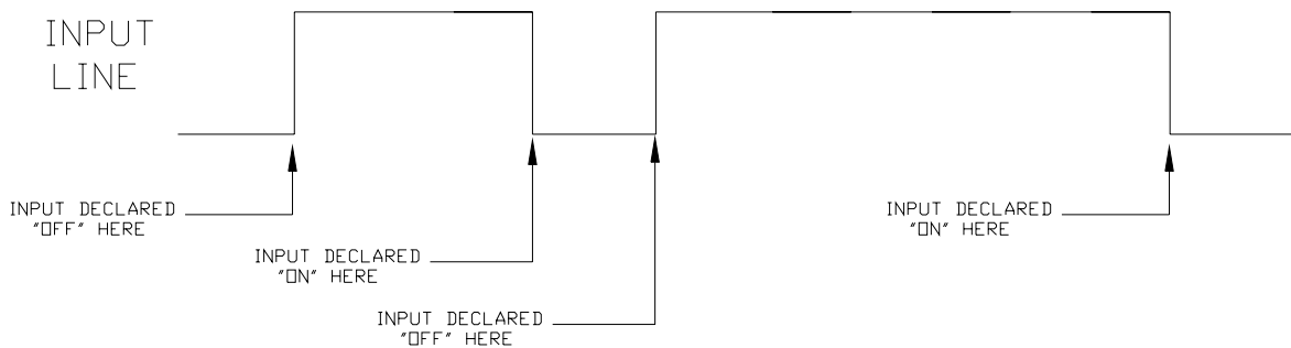
Figure-8 Example of Edge Detection Process
