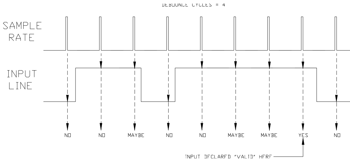
Figure-5 Example of the Debouncing Process
