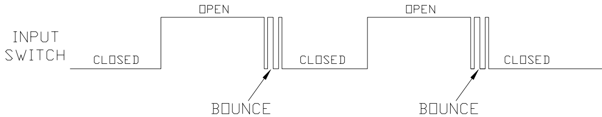
Figure-4 Example of Switch Bounce
